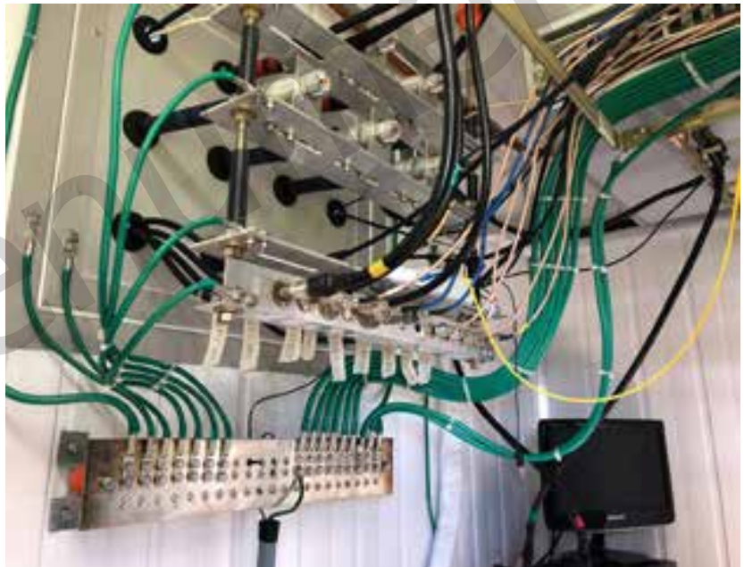
Antenna panel.
